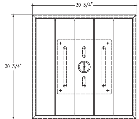
TOP VIEW 1052
