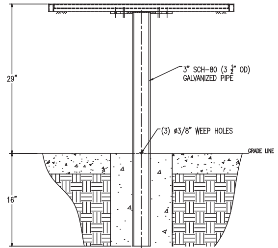
ELEVATION VIEW
