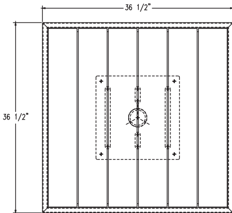
TOP VIEW 1042
