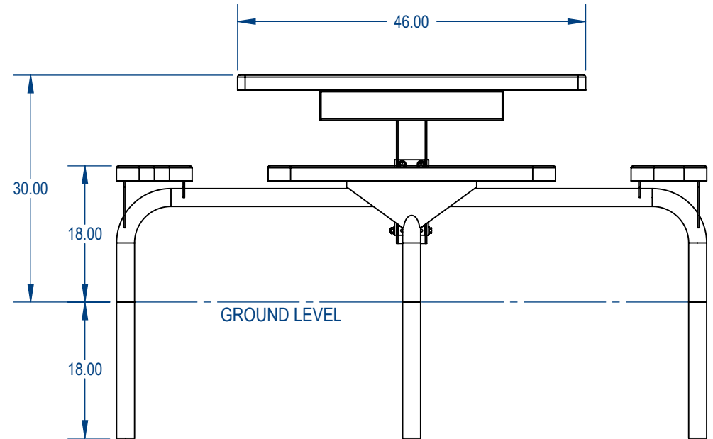
SIDE VIEW
